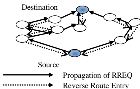
Figure 4.2 Propagation of an AODV RREQ and establishment of the reverse routes
