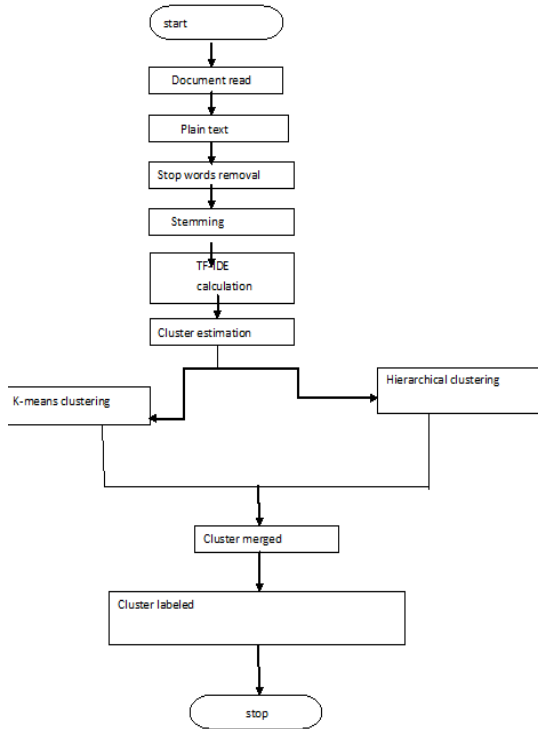
Figure 1 : System Flowchart.
